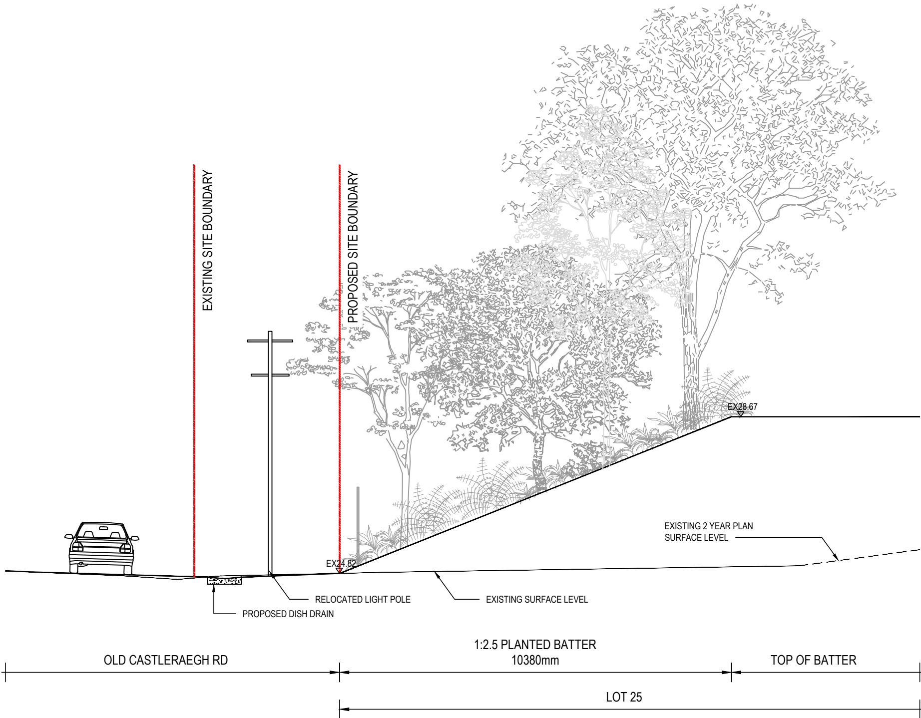
1 SECTION 1 1:100
