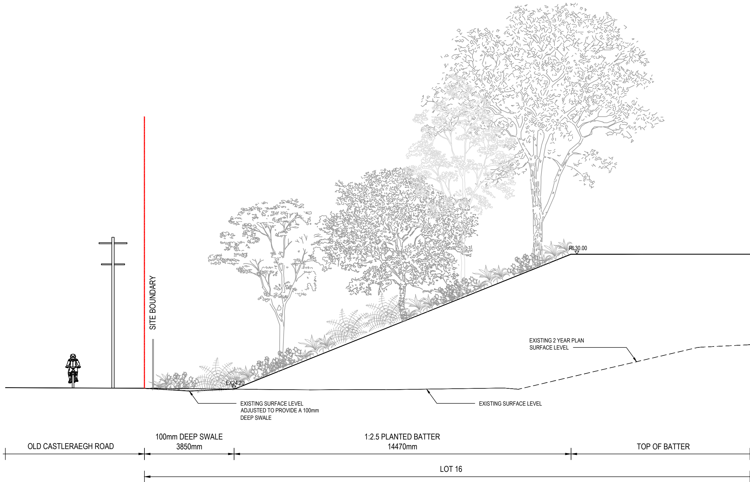
2 SECTION 2 1:100
